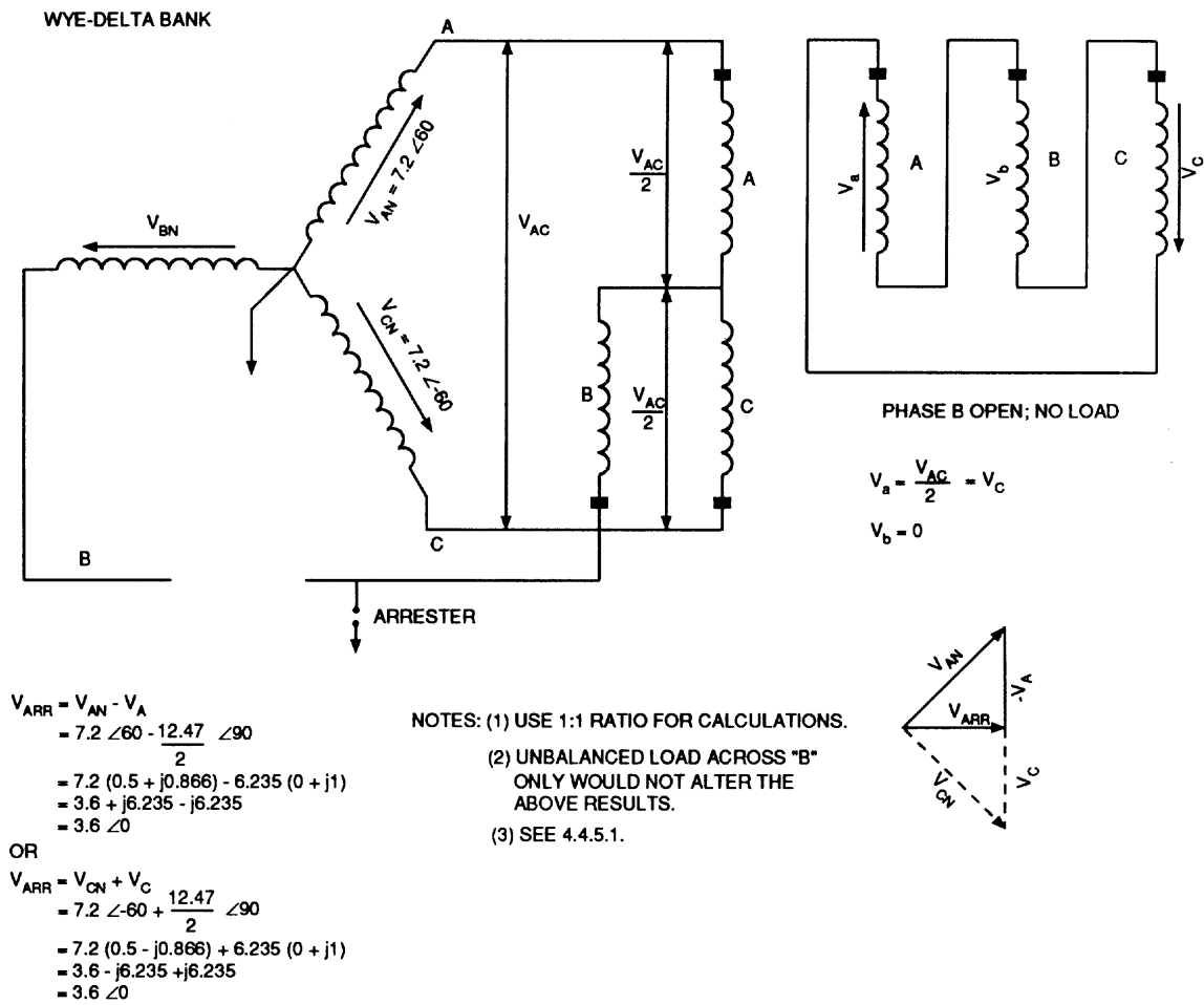
Figure E.2—Open primary
