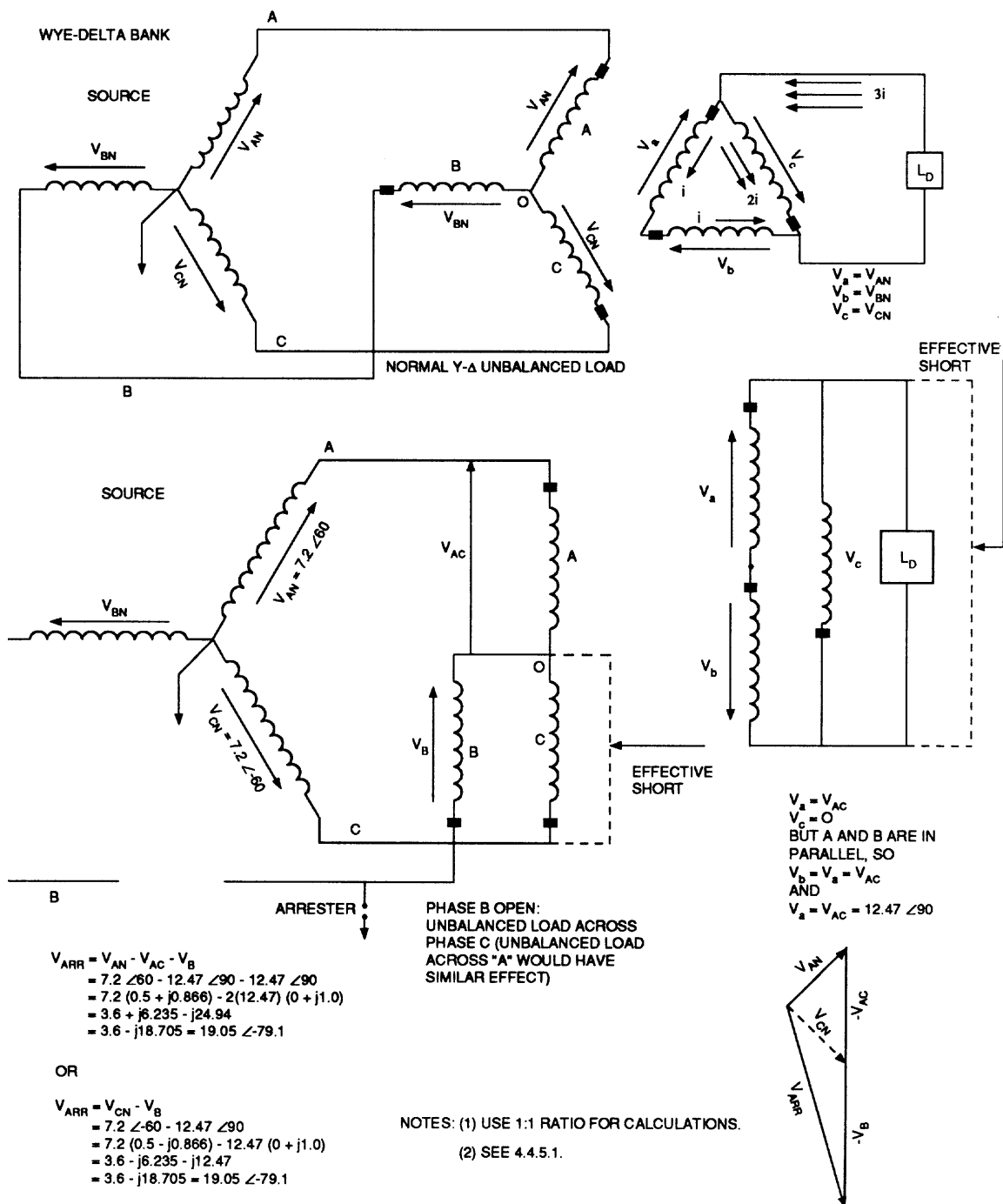
Figure E.1—Shorted secondary
