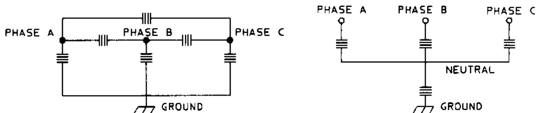
Figure 8—Phase-to-phase protection
