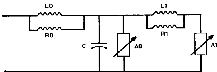
Figure G.1 — Frequency-dependent model
